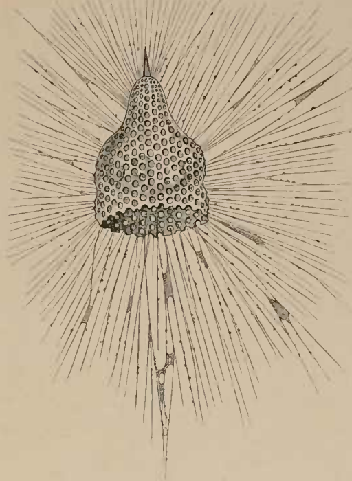
FIG. XV.— Eucyrtidium cranioides , Hæck; \times 150 ; one of the Monopylæa. Entire animal as seen in the living condition. The central capsule is hidden by the bee-hive-shaped siliceous shell within which it is lodged.
