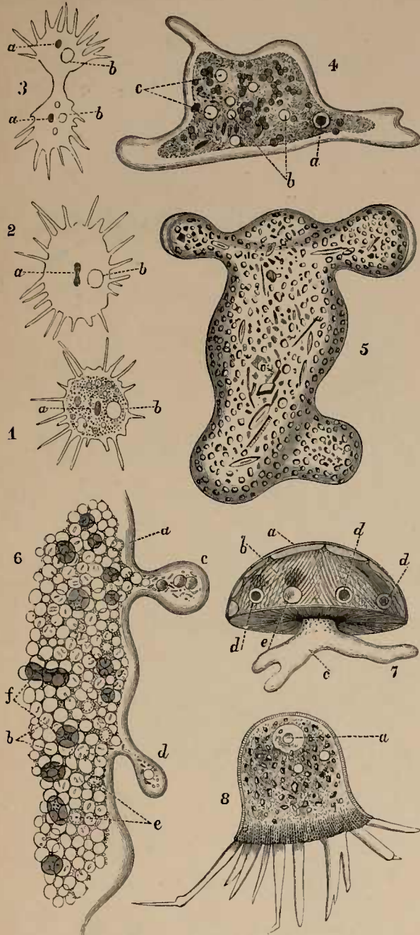
FIG. IV.—Various Lobosa. 1, 2, 3. Dactylosphaera ( Amoeba ) polytipodia , M. Schultze, in three successive stages of division; the changes indicated occupied fifteen minutes. a , nucleus; b , contractile vacuole (copied from F. E. Schultze, in Archiv. Mikrosk. Anat. ). 4. Amoeba princeps , Ehr. (after Auerbach). a , nucleus; b , c , vacuoles (one or more contractile; the shaded granules are food-particles). 5. Pelomyxa palustris , Greeff (after Greeff), an example with comparatively few food-particles (natural size \frac{1}{3} th inch in length). 6. Portion of a Pelomyxa more highly magnified. a , clear superficial zone of protoplasm (so-called "exoplasm"); b , vacuoles, extremely numerous; c , lobose pseudopodium; d , a similar pseudopodium; e , nuclei; f , "refractive bodies" (reproductive?); scattered about in the protoplasm are seen numerous cylindrical crystals. 7. Arcella vulgaris , Ehr. a , shell; b , protoplasm within the shell; c , extended protoplasm in the form of lobose pseudopodia; d , nuclei; e , contractile vacuole; the dark bodies unlettered are gas vacuoles. 8. Cochliopodium pellucidum , Hert. and Less. a , nucleus surrounded by a hyaline halo sometimes mistaken for the nucleus, whilst the latter is termed nucleolus.
