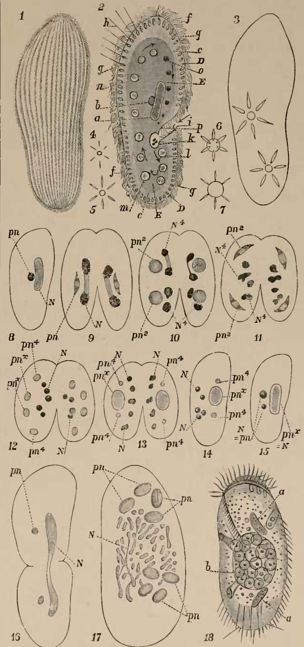
FIG. XXV. Ciliata (conjugation, etc.). 1. Surface view of Holotrichous Ciliate, showing the disposition of the cilia in longitudinal rows. 2.
