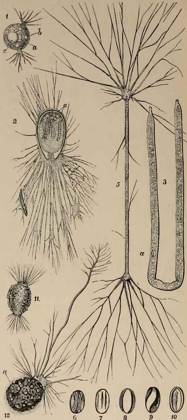
FIG. IX.—Gromiidea (Reticularia membranosa). 1. Diplophrys Archeri , Barker. a, nucleus; b, contractile vacuoles; c, the yellow oil-like body. Moor pools, Ireland. 2. Gramia oviformis , Duj. a, the numerous nuclei; near these the elongated bodies represent ingested diatoms. Freshwater. 3. Shephardella tenuiformis , Siddall ( Quart. Jour. Micr. Sci. , 1880); \times 30 diameters. Marine. The protoplasm is retracted at both ends into the tubular case. a, nucleus. 4. Shephardella tenuiformis ; \times 15 ; with pseudopodia fully expanded. 5-10. Varying appearance of the nucleus as it is carried along in the streaming protoplasm within the tube. 11. Amphitrema Wrightianum , Archer, showing membranous shell encrusted with foreign particles. Moor pools, Ireland. 12. Diaphorophodon mobile , Archer. a, nucleus. Moor pools, Ireland.
