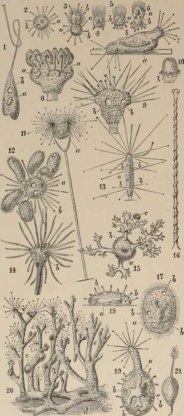
FIG. XXVI.—Acinetaria. 1. Rhyncheta cyclopium , Zenker. a, nucleus; b, contractile vacuole; only a single tentacle, and that suctorial; × 150. Parasitic on Cyclops. 2. Sphaerophrya urostyla , Maupas; normal adult; × 200. a, nucleus; b, contractile vacuole. Parasitic in Urostyla . 3. The same dividing by transverse fission, the anterior moiety with temporarily developed cilia. a, nucleus; b, contractile vacuole. 4, 5, 6. Sphaerophrya stentorea , Maupas; × 200. Parasitic in Stentor , and at one time mistaken for its young. 7. Trichophrya epistylidis , Cl. and L.; × 150. a, nucleus; b, contractile vacuole. 8. Hemiofrya gemmipara , Hertwig; × 400. Example with six buds, into each of which a branch of the nucleus a is extended. 9. The same species, showing the two kinds of tentacles (the suctorial and the pointed) and the contractile vacuoles b. 10. Ciliated embryo of Podophrya Steinitz , Cl. and L.; × 300. 11. Acineta grandis , Saville Kent; × 100; showing pedunculated lorica, and animal with two bunches of entirely suctorial tentacles. a, nucleus. 12. Sphaerophrya magna , Maupas; × 300. It has seized
