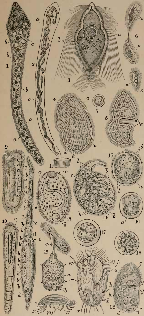
FIG. XXIV. Ciliata.—1. Ophaltnopsis septiole , Foett.; a parasitic Holotrichous mouthless Ciliate from the liver of the Squid. a , nuclei; b , vacuoles (non-contractile). 2. A similar specimen treated with picricarmin, showing a remarkably branched and twisted nucleus; a , in place of several nuclei. 3. Trichonympha agilis , Leidy; parasitic in the intestine of the Termites (White Ants); \times 600 . a , nucleus; b , granules (food?). 4. Opalina ranarum , Purkinje; a Holotrichous mouthless Ciliate parasitic in the Frog's rectum; adult; \times 100 . a , the numerous regularly dispersed nuclei. 5. The same; an individual in process of binary fission. a , nuclei. 6. The same; the process of fission has now reduced the individuals to a relatively small size. 7. Smallest fission-produced fragment encysted, expelled from the Frog in this state and swallowed by Tadpoles. 8. Young uninucleate individual which has emerged from the cyst within the Tadpole, and will now multiply its nuclei and grow to full size before in turn undergoing retrogressive fission. 9. Anoplophrya naidos , Duj.; a mouthless Holotrichous Ciliate parasitic in the worm Nais; \times 200 . a , the large axial nucleus; b , contractile vacuoles. 10. Anoplophrya prolifera , C. and L.; from the intestine of Clitello. Remarkable for the adhesion in a metameric series
