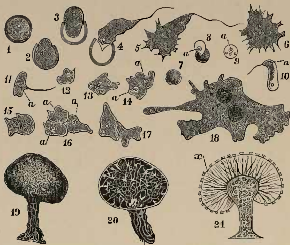
FIG. 111.—Mycetozoa (after De Bary). 1-6. Germination of spore (1) of Trichea varia , showing the emerging "flagellula" (4, 5), and its conversion into an "amœbula" (6). 7-18. Series leading from spore to plasmodium phase of Chondrioderma difforme :—7, spore; 10, flagellula; 12, amœbula; 14, apposition of two amœbulae; 15-17, fusions; 18, plasmodium. 19, 20. Spore-fruit (cyst) of Physarum leucophæum , Fr. ( \times 25 ), the former from the surface, the latter in section with the spores removed to show the sustentacular network or capillitium. 21. Section of the spore-cyst of Didymium squamosum , with the spores removed to show the radiating capillitium x and the stalk.
